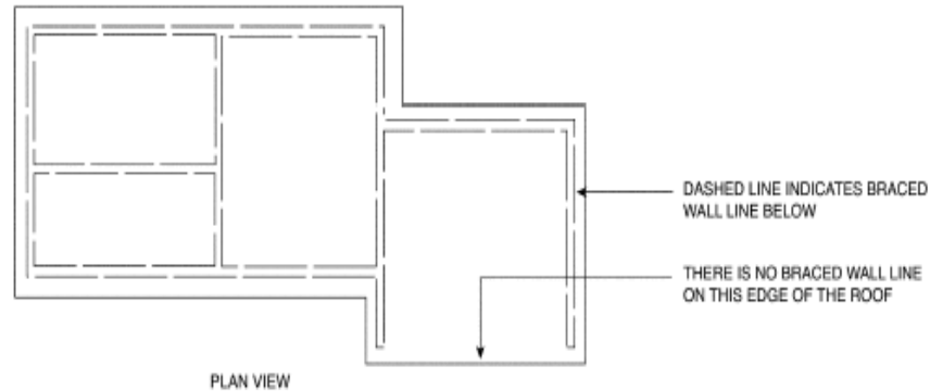
Figure 2308.12.6(3)
