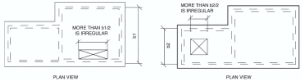
Figure 2308.12.6(8)
